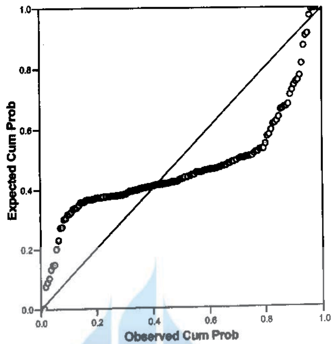
Normal P-P Plot of PER
