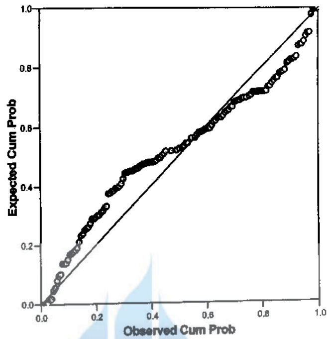
Normal P-P Plot of ROI
