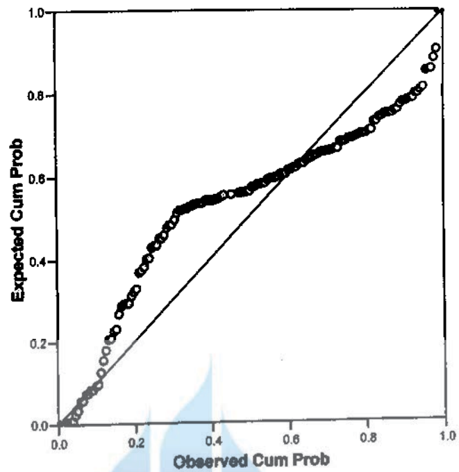
Normal P-P Plot of ROE
