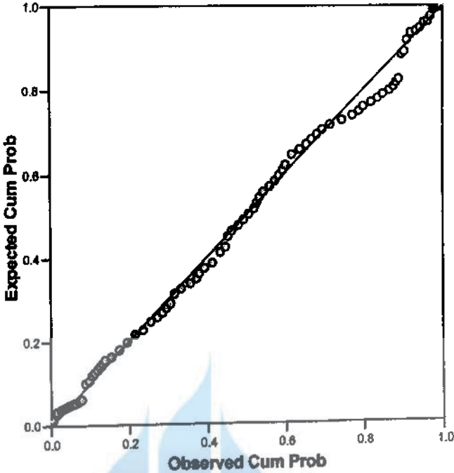
Normal P-P Plot of LEVERAGE
