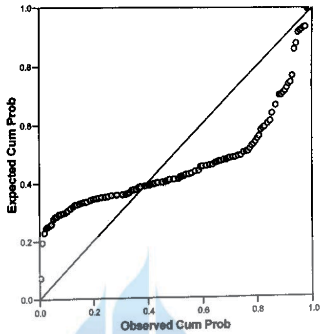
Normal P-P Plot of PBV
