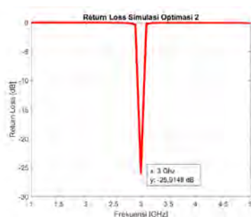
Gambar 5. Return Loss Hasil Optimasi Ground Plane
