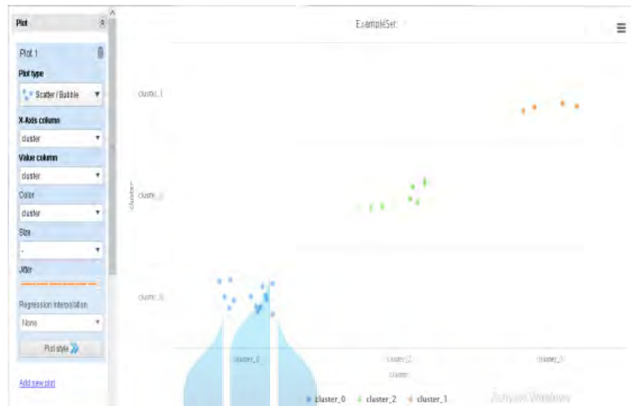
Gambar 12. Tampilan Scatter
