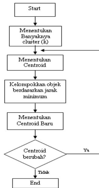
Gambar 3. Flowchart K-Means [6]
