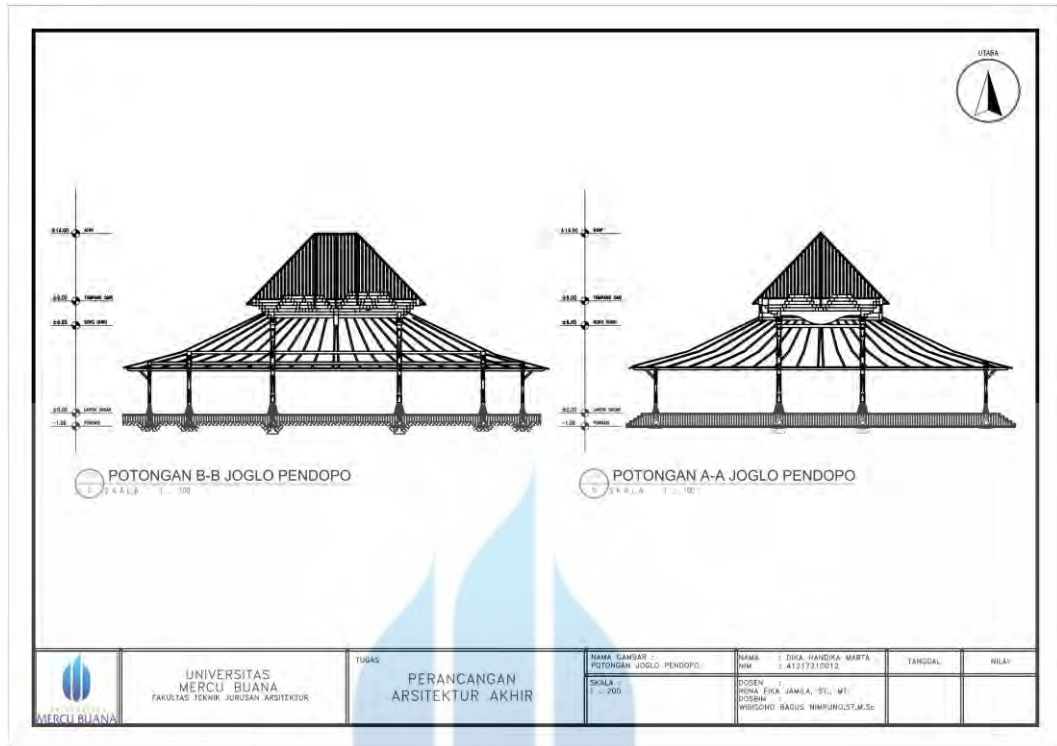
Lampiran 18 Potongan B-B Joglo Pendopo
