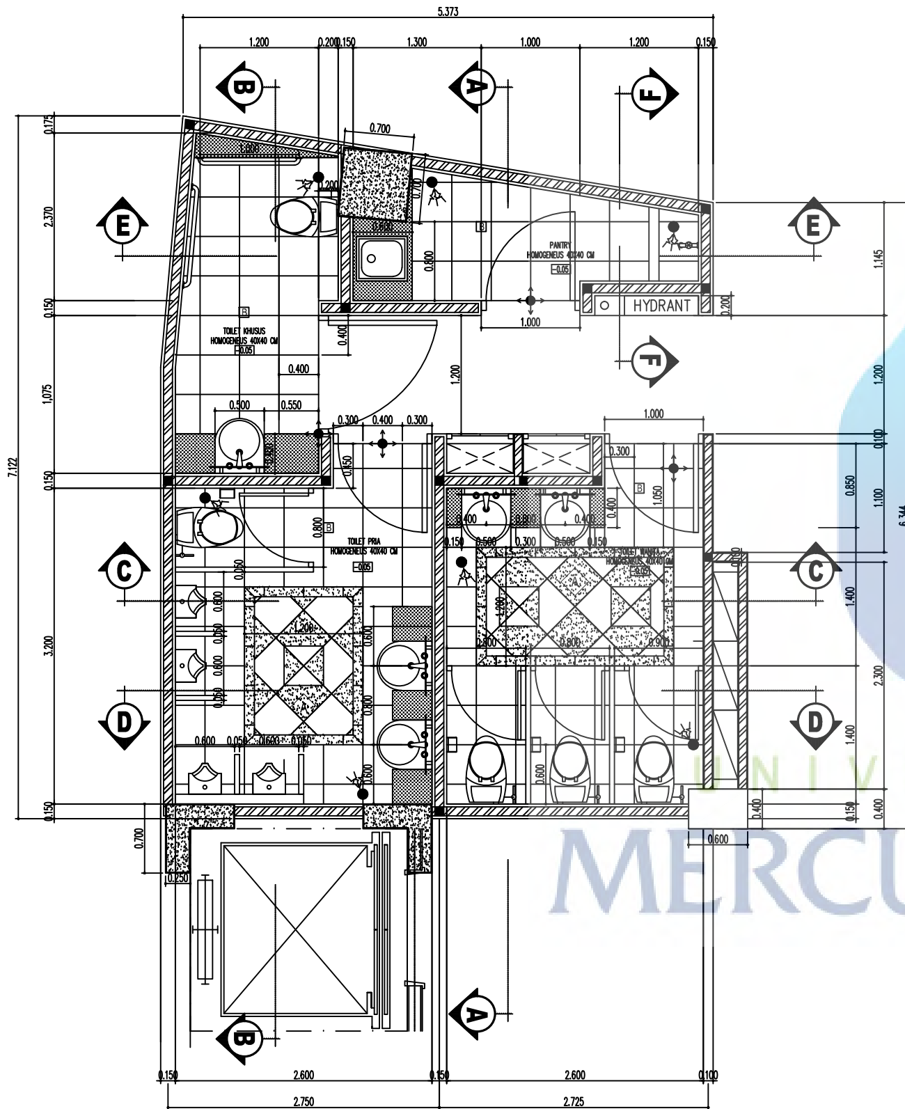
DENAH TOILET SKALA 1:50
