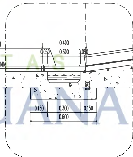
DETAIL A SKALA 1 : 10
