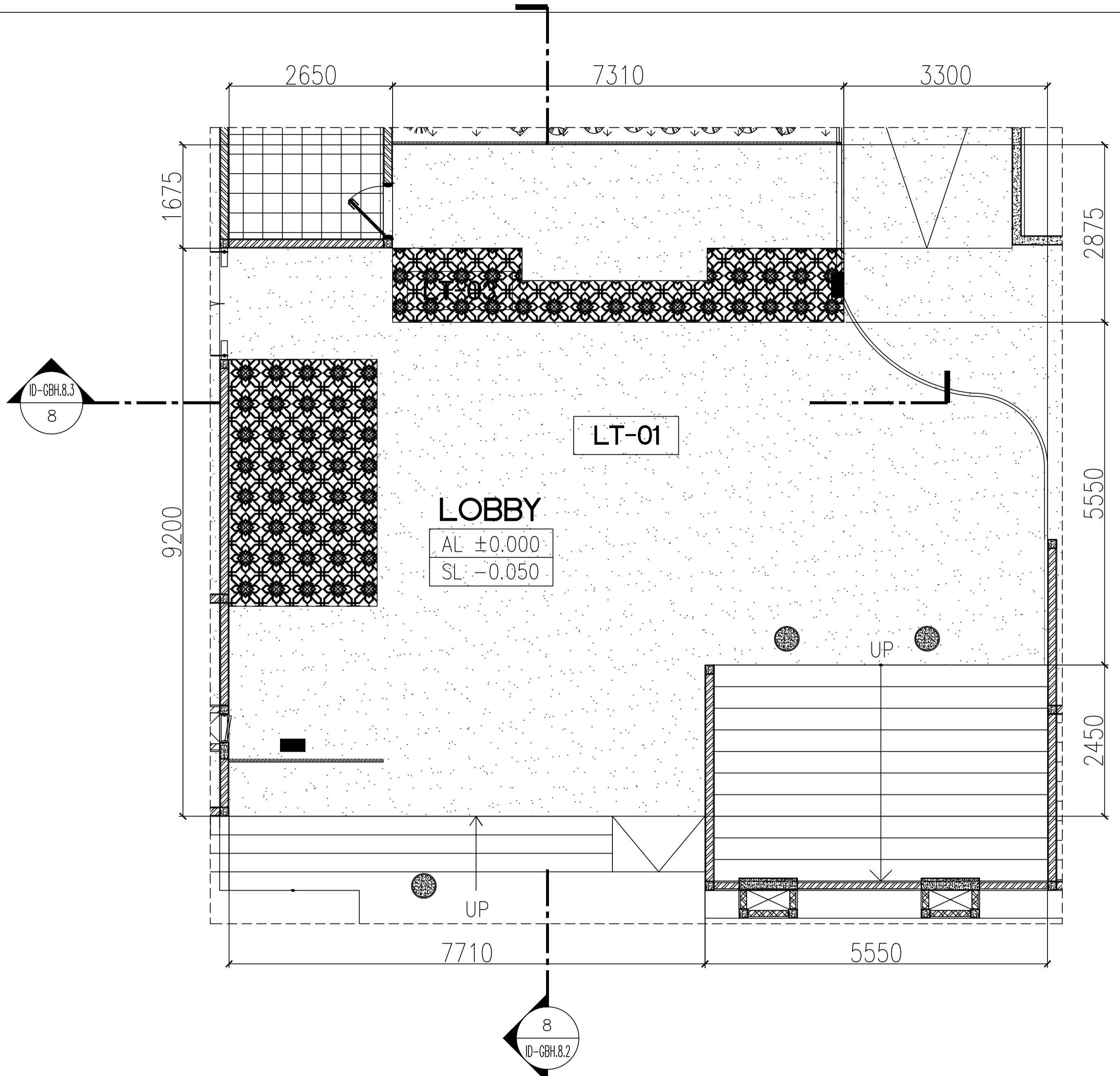
GROUND FLOOR FLOOR RESTAURANT PLAN SCALE 1: 50 3 ID-GBH.3.1
