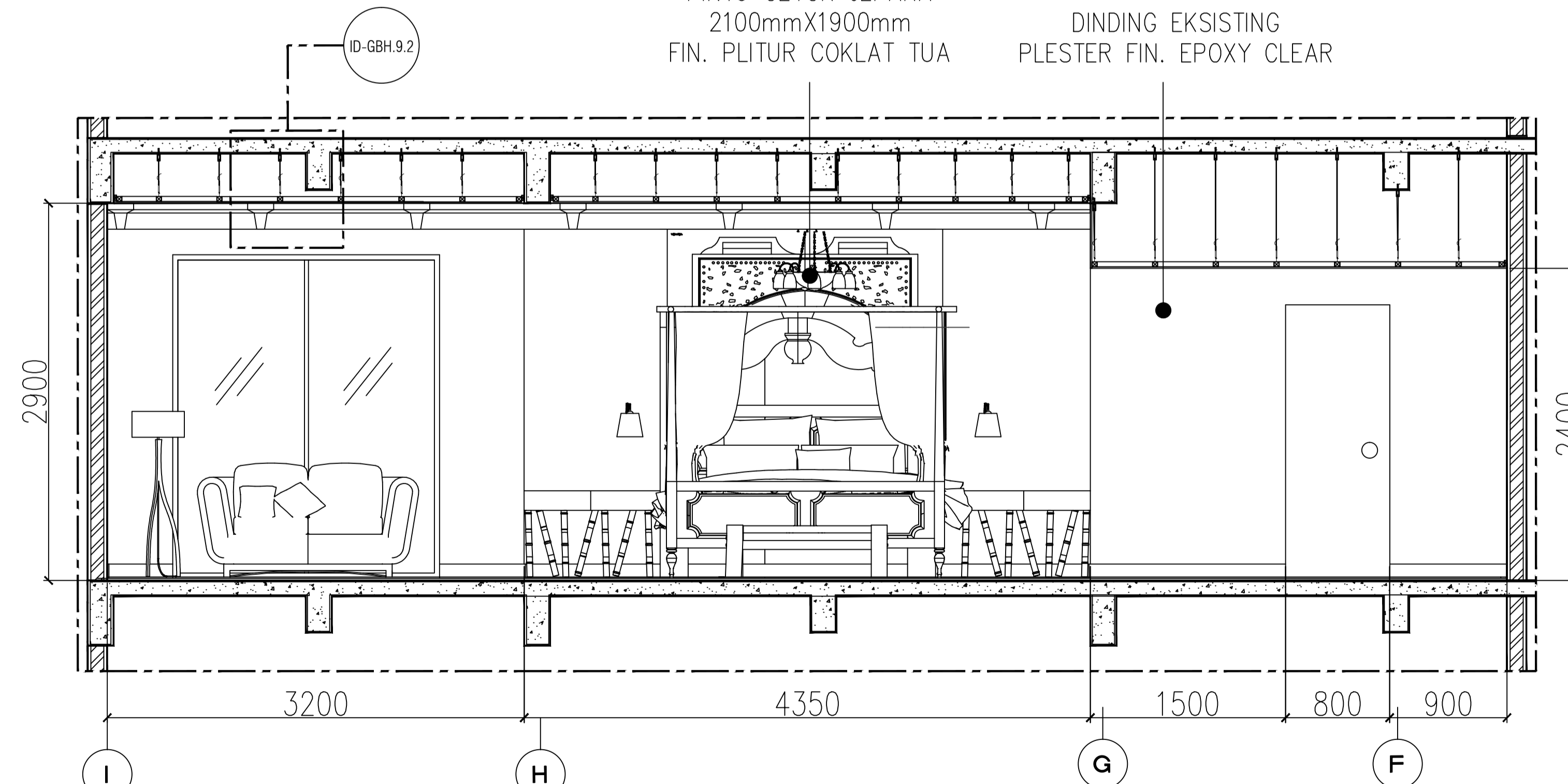
8 ID-GBH.8.6 GROUND FLOOR POTONGAN G-G SCALE 1:30
