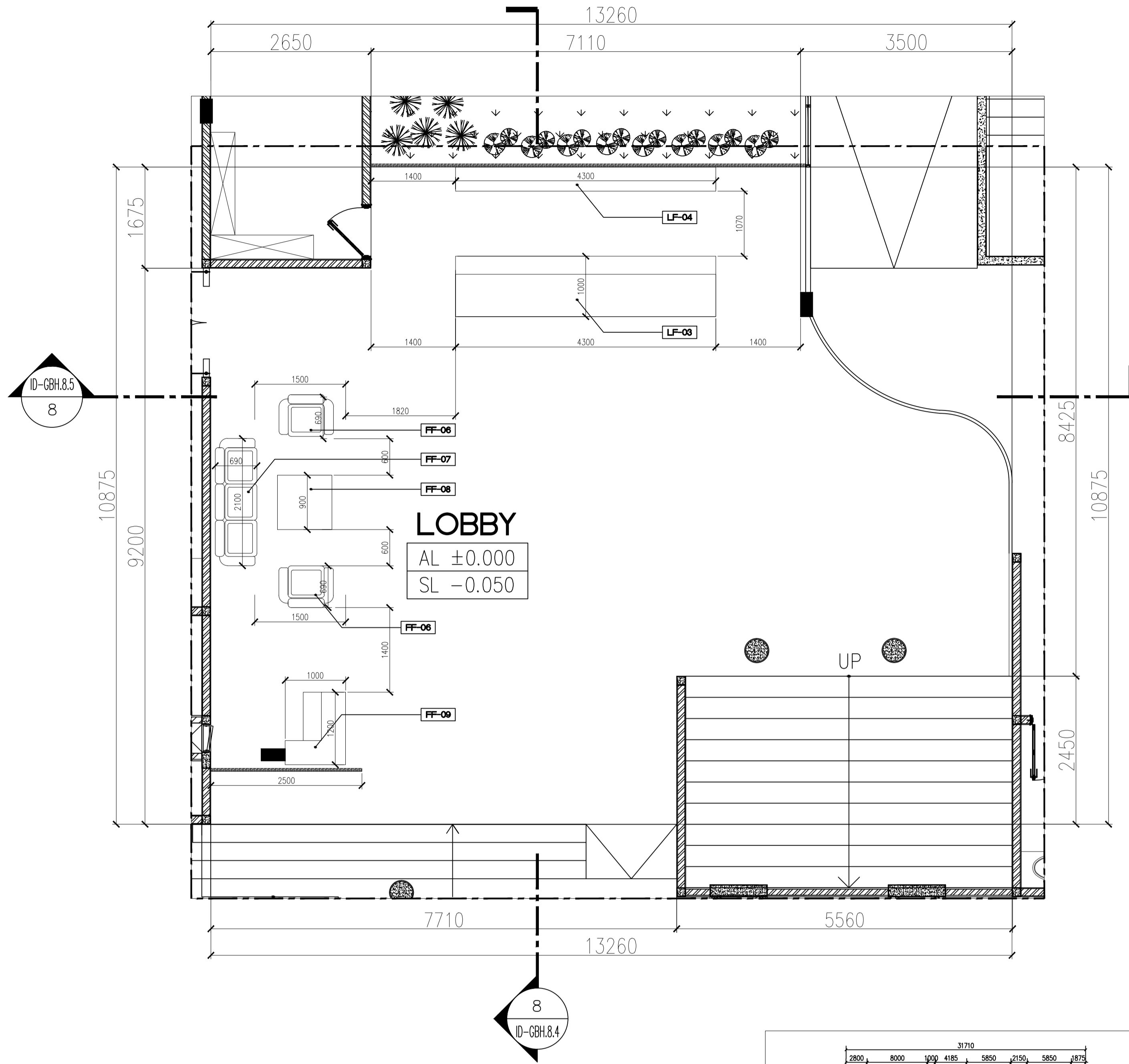
2 ID-GBH.2.1 GORUND FLOOR RECEPTIONIST LAYOUT PLAN SCALE 1:50
