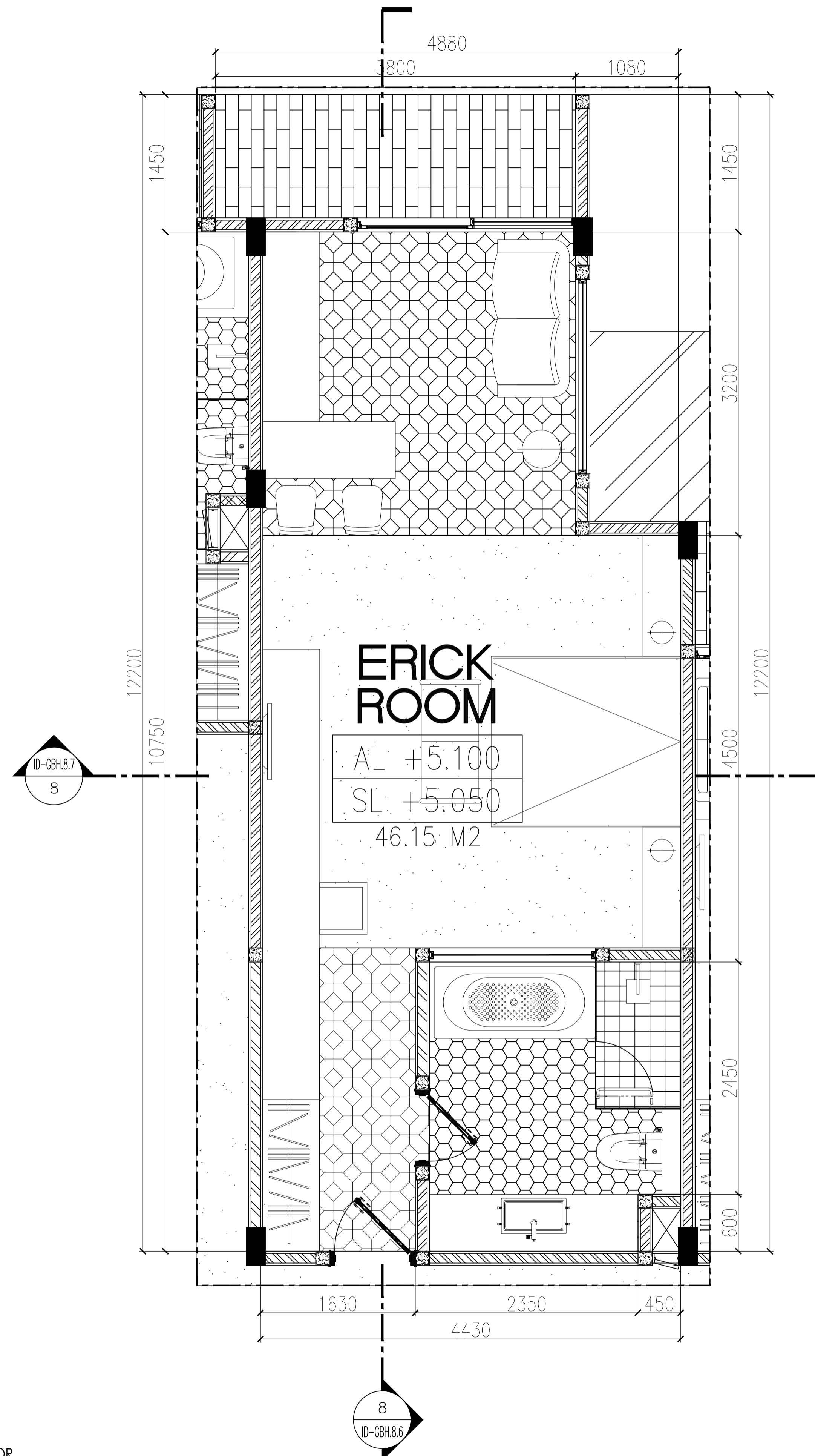
1 ID-GHB.1.8 THIRD FLOOR ERICK ROOM LAYOUT PLAN SCALE 1:30
