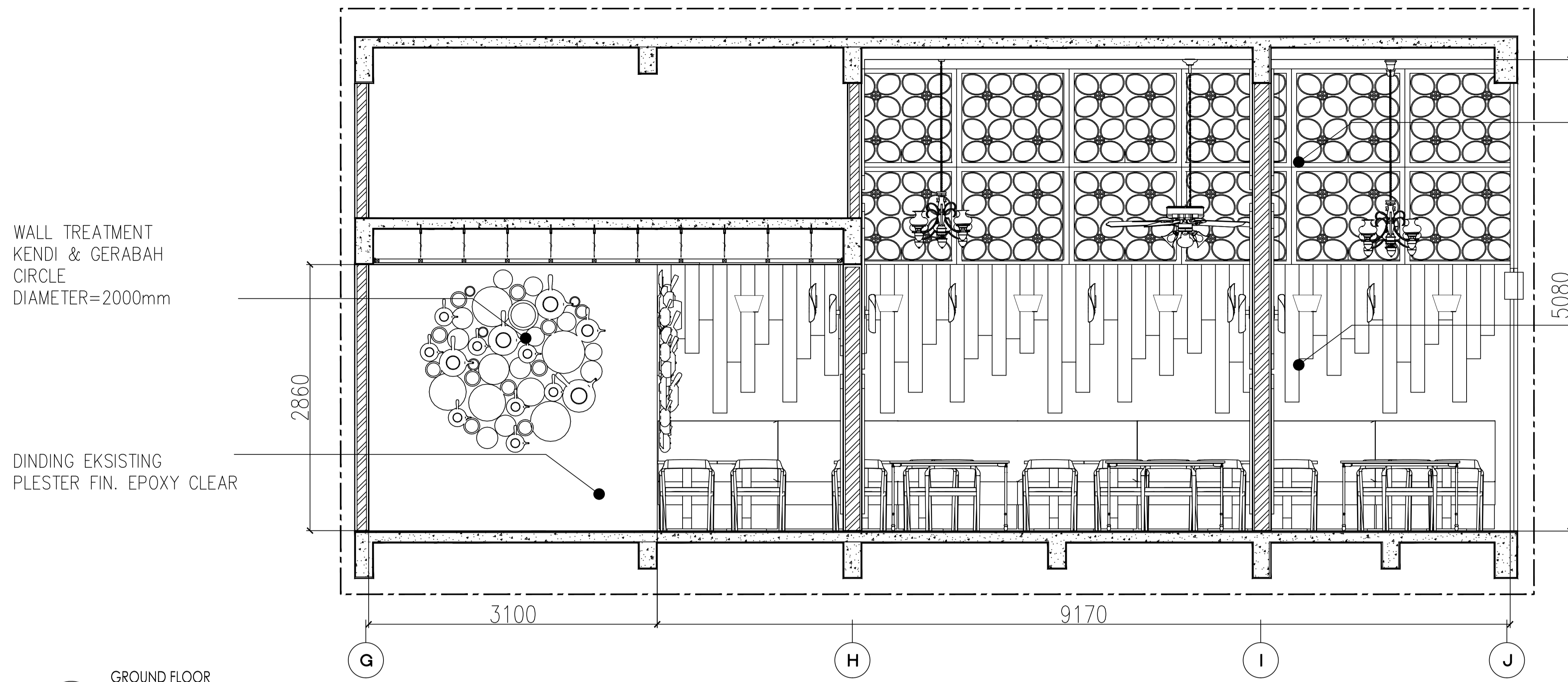
8 ID-GBH.8.0 GROUND FLOOR POTONGAN A-A SCALE 1:30
