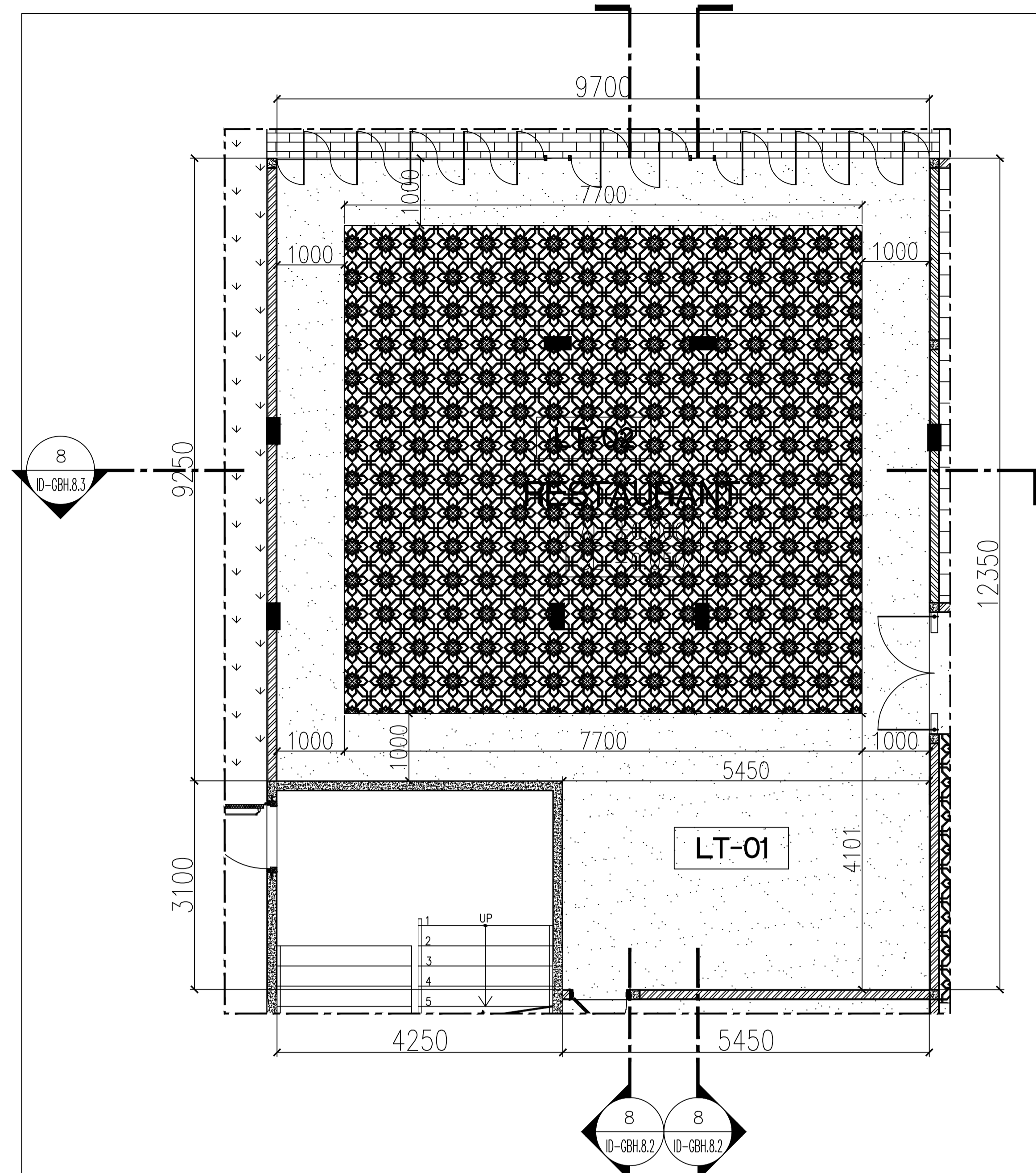
GROUND FLOOR FLOOR RESTAURANT PLAN SCALE 1: 50 3 ID-GBH.3.1
