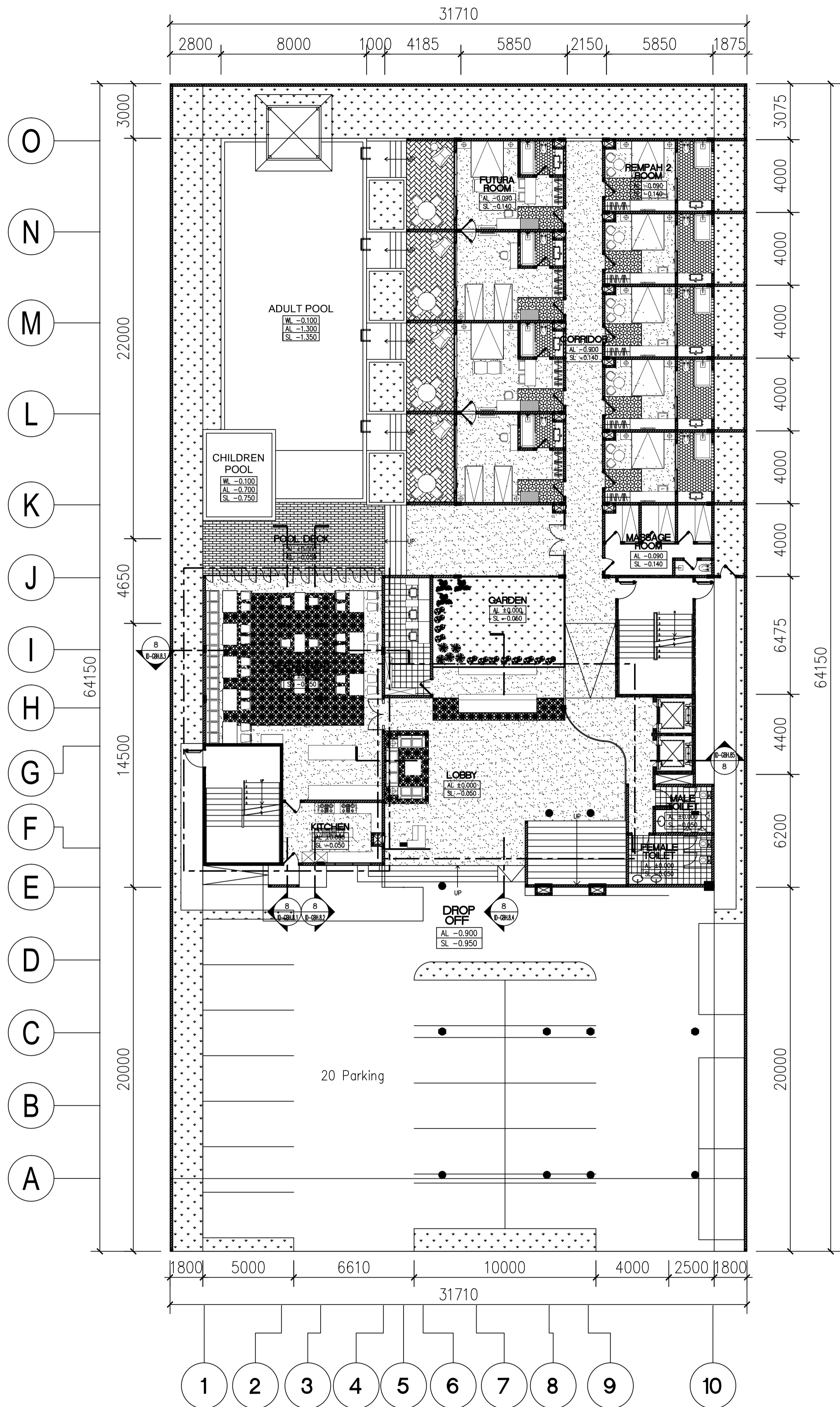
1 ID-GHB.1.0 GROUND FLOOR LAYOUT PLAN SCALE 1:150
