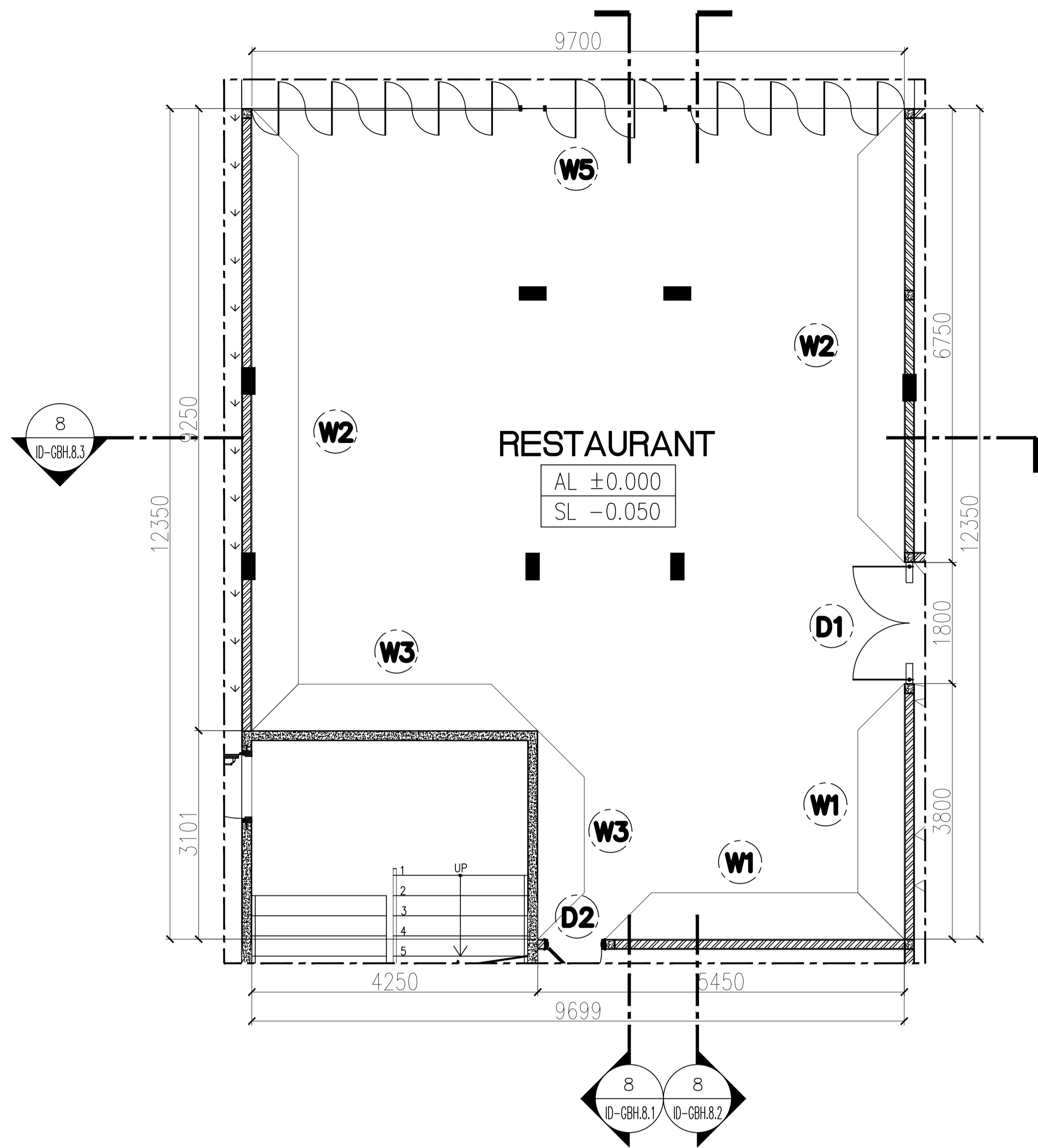
7 ID-GHB.7.0 GROUND FLOOR WALL TREATMENT PLAN SCALE 1:50
