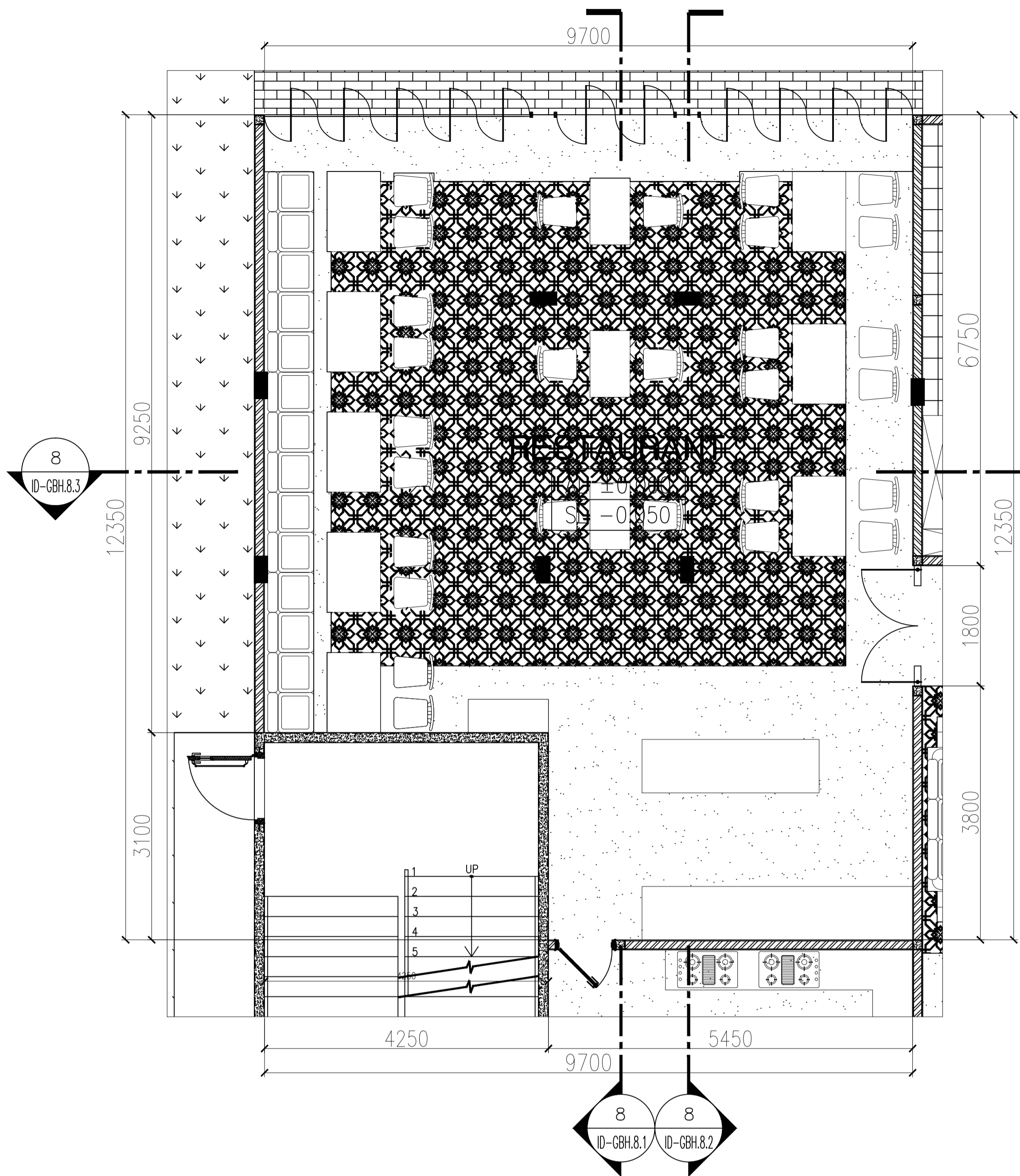
1 GORUND FLOOR RESTAURANT LAYOUT PLAN ID-GBH.1.6 SCALE 1:50
