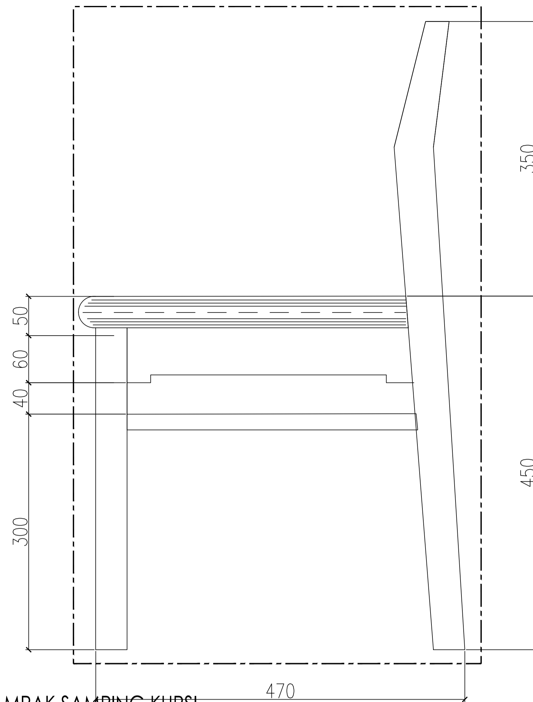
11 ID-GHB.11.1 TAMPAK SAMPING KURSI SCALE 1:3
