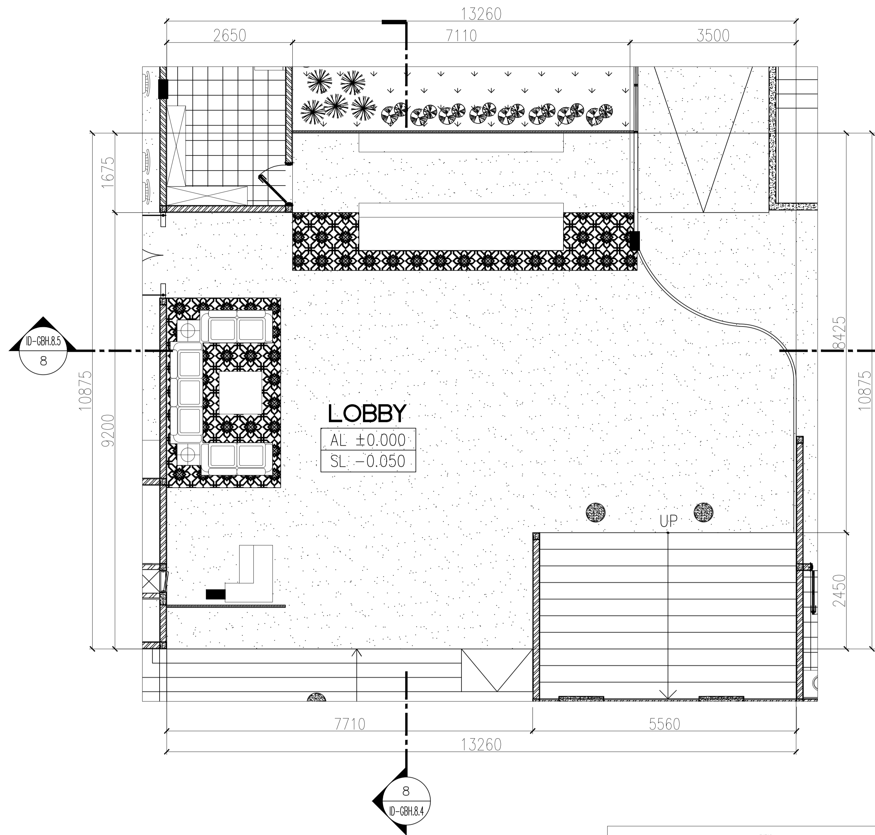
1 GORUND FLOOR RECEPTIONIST LAYOUT PLAN ID-GBH.1.7 SCALE 1:50
