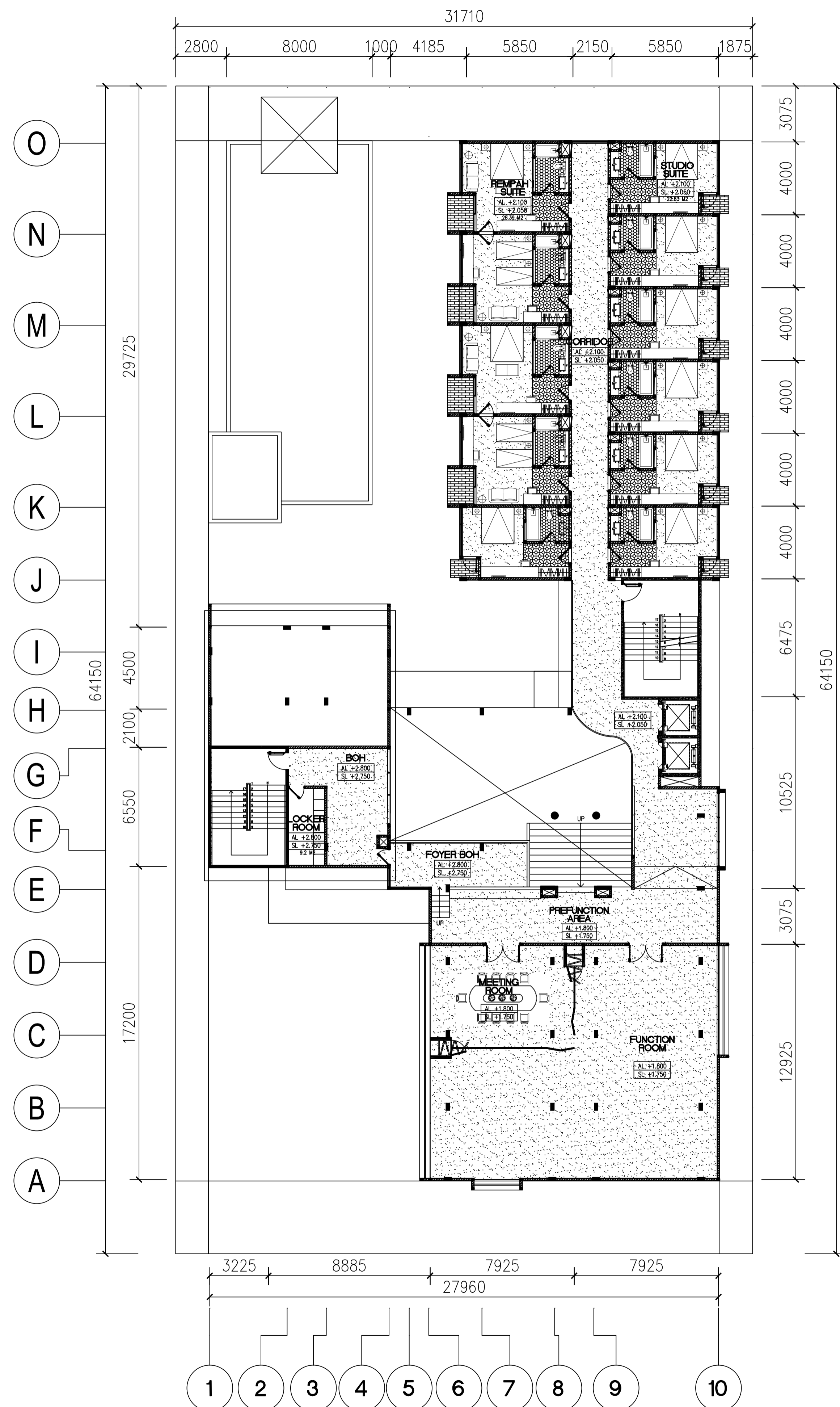
1 ID-GHB.1.1 FIRST FLOOR LAYOUT PLAN SCALE 1:150
