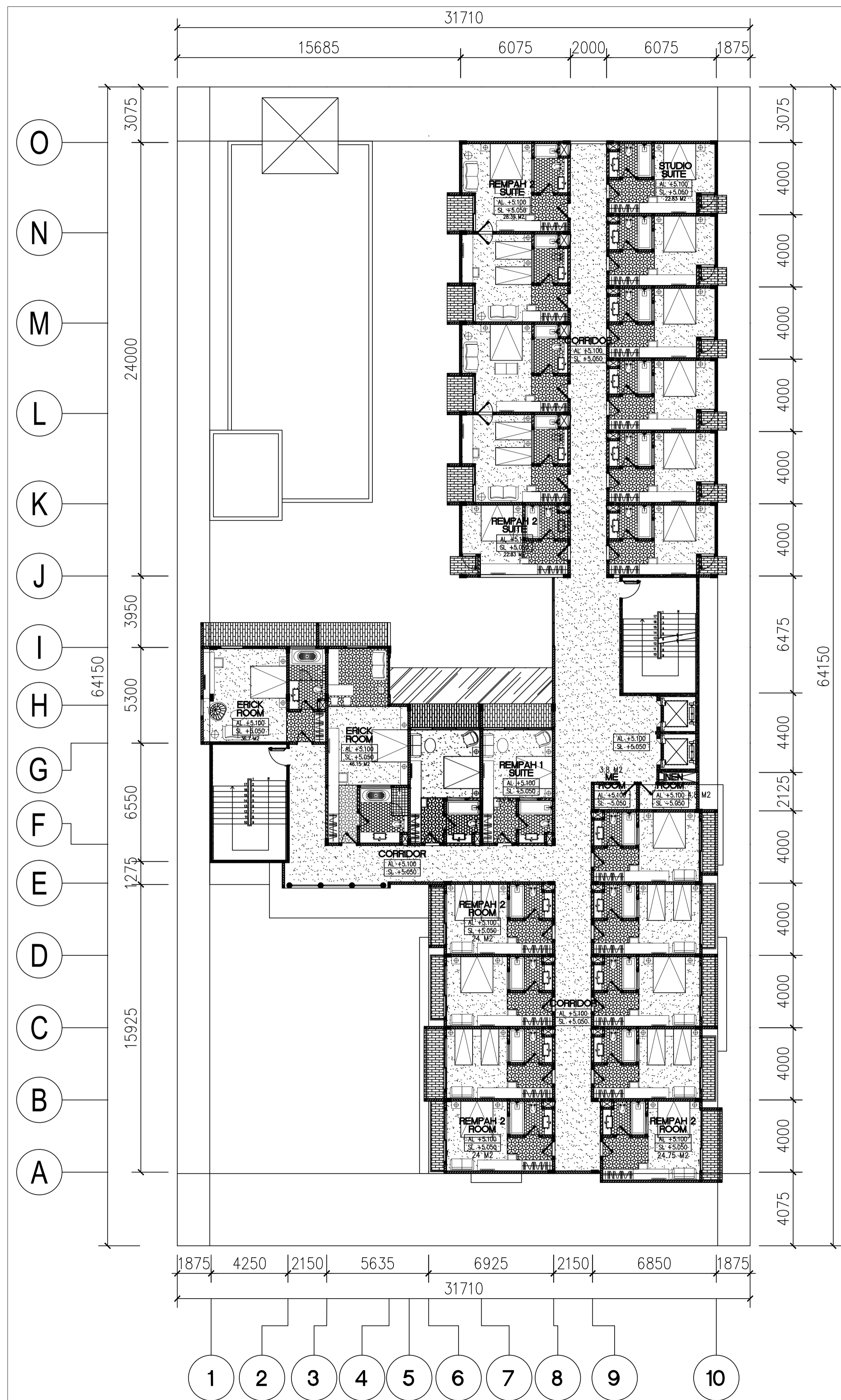
1 ID-GHB.1.4 FOURTH FLOOR LAYOUT PLAN SCALE 1:150
