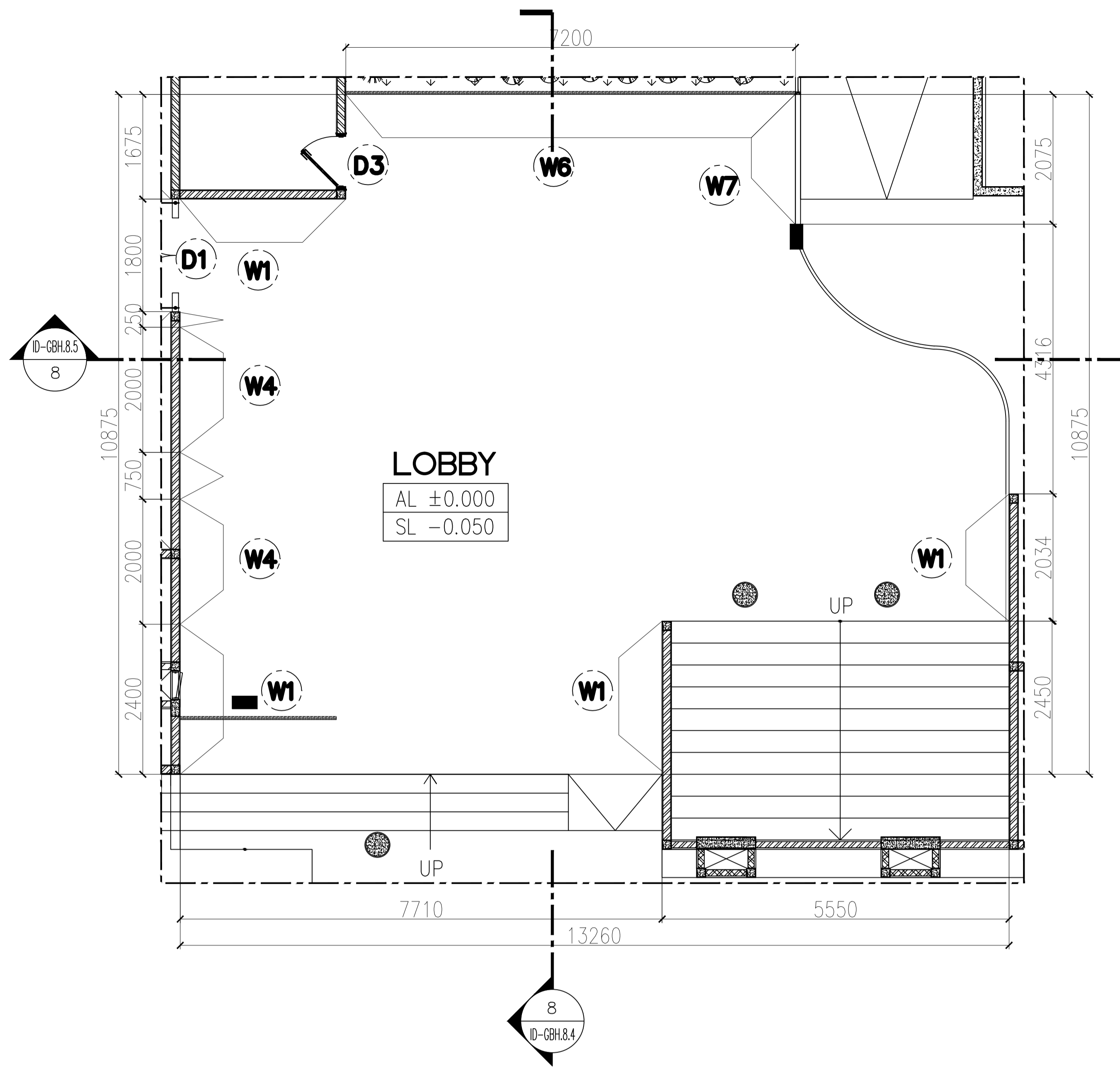
7 ID-GHB.7.1 GROUND FLOOR WALL TREATMENT PLAN SCALE 1:50
