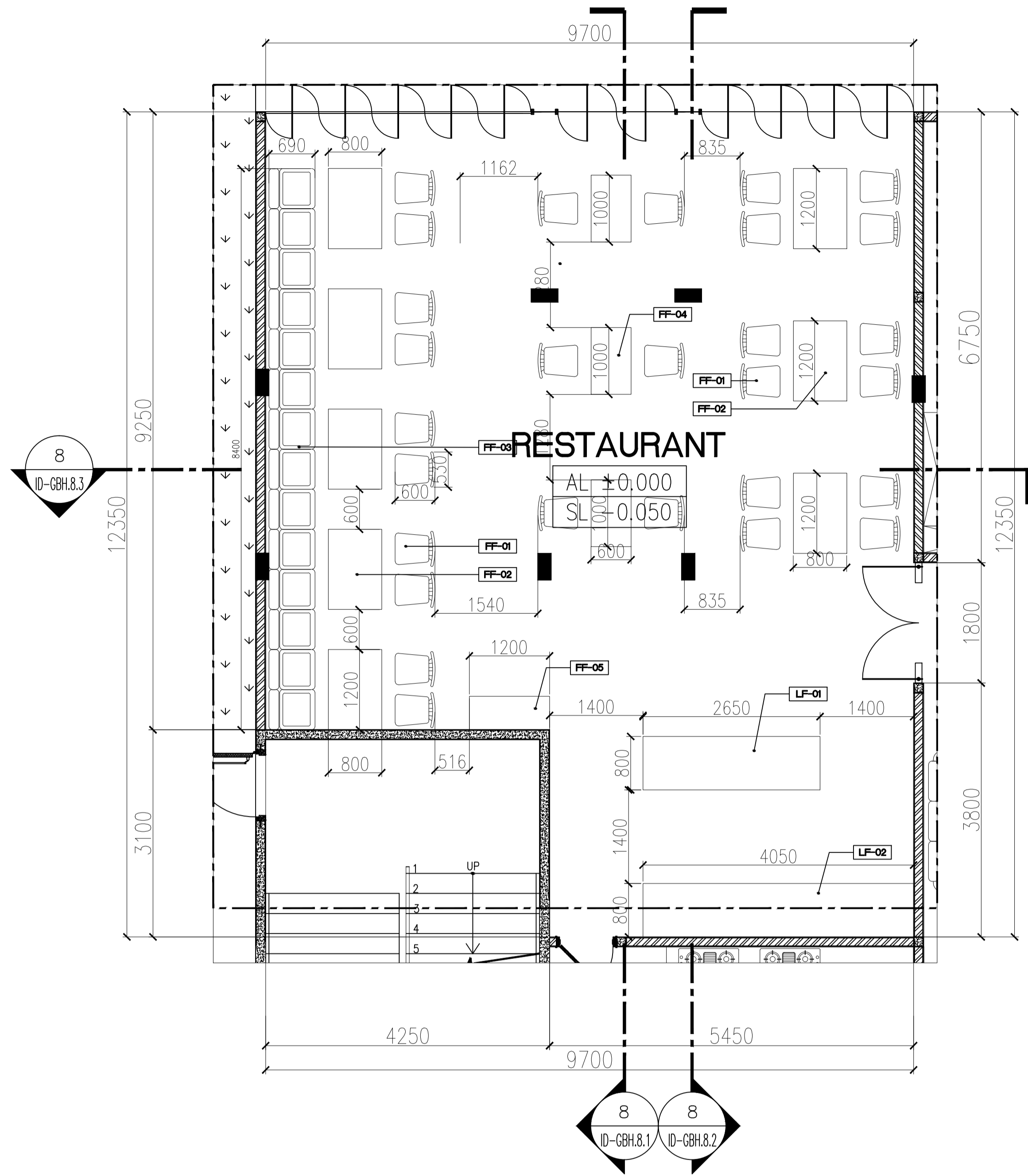
2 ID-GBH.2.0 GORUND FLOOR RESTAURANT LAYOUT PLAN SCALE 1:50
