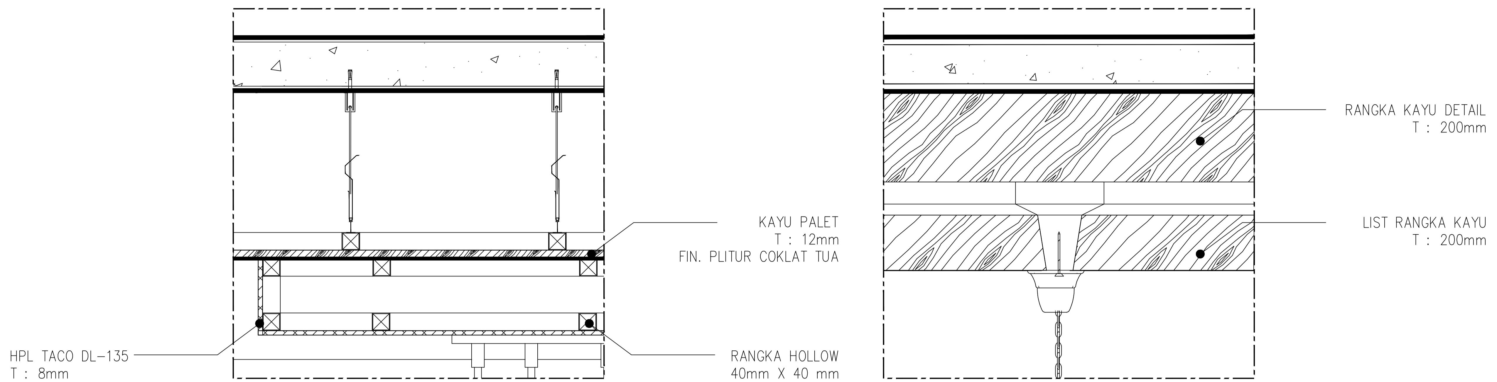
9 ID-GBH.9.0 SCALE 1:5 DETAIL PLAFON BUFFET
