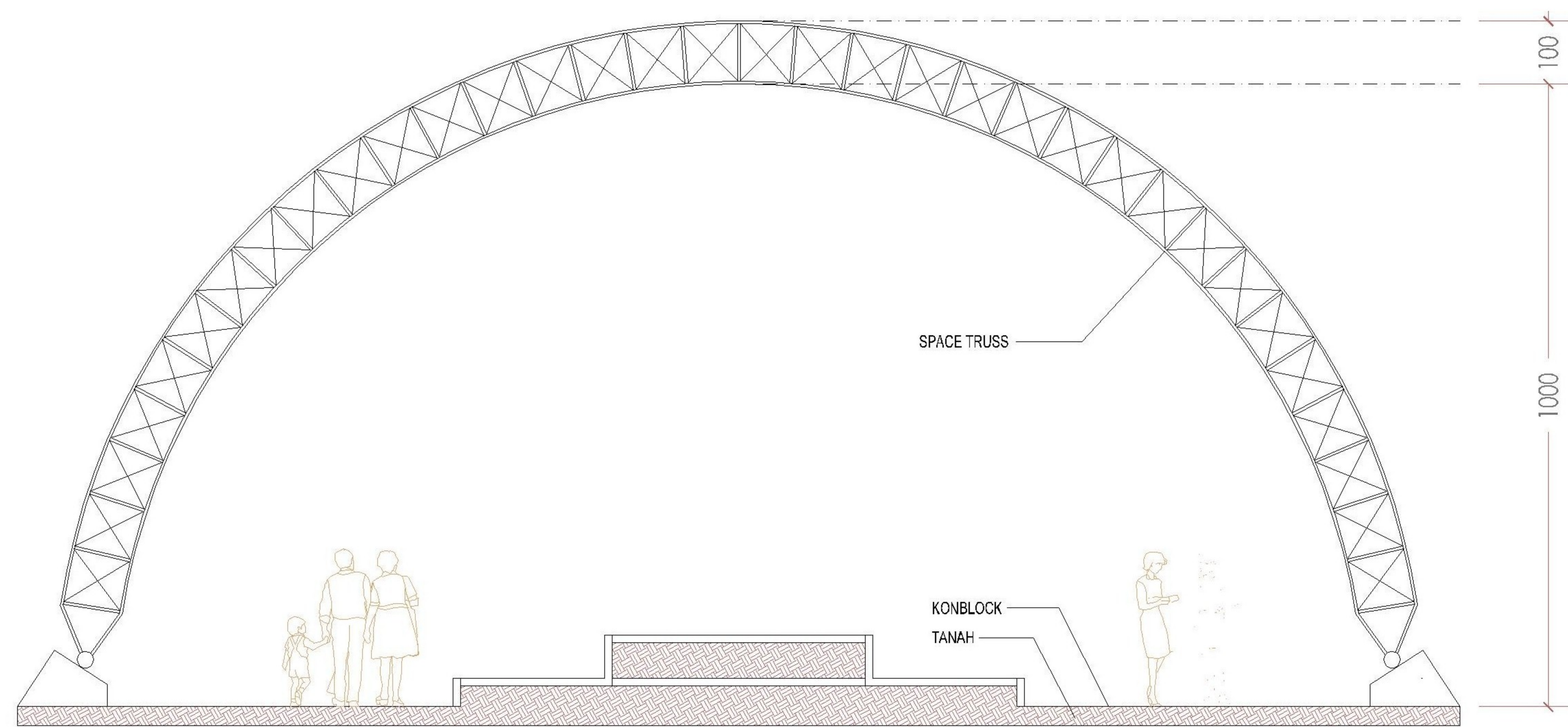
DETAIL POTONGAN - D
