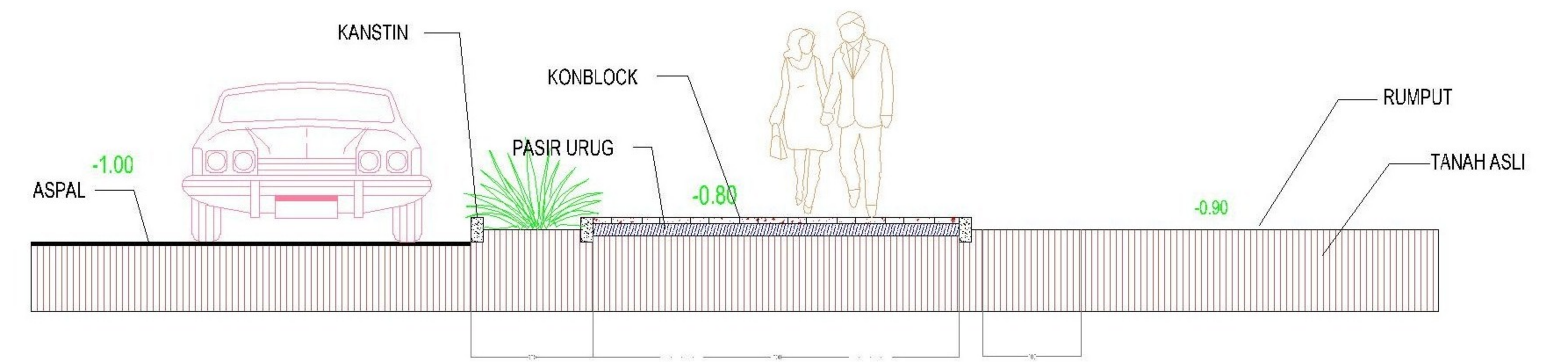
DETAIL POTONGAN - E
