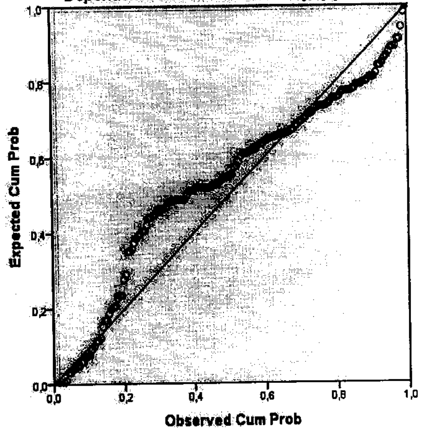
Normal P-P Plot of Regression Standardized Residual Dependent Variable: Prestasi Kerja (Y)
